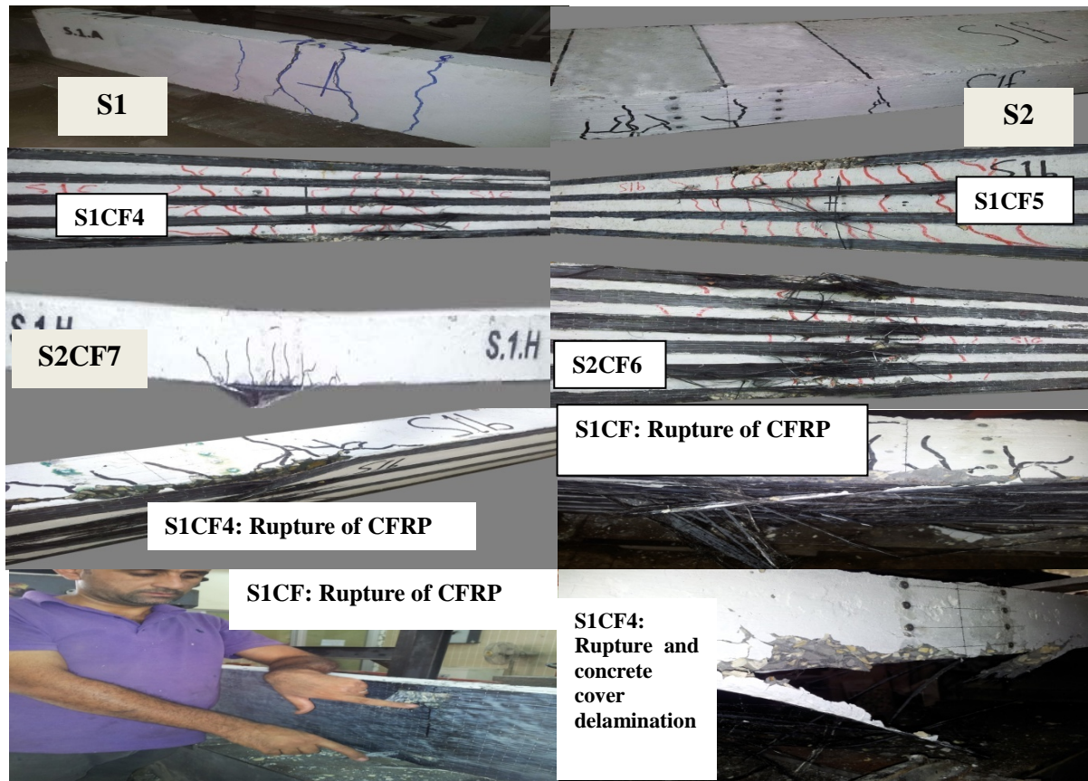
Fig. (7): Crack Patterns and Failure modes of strengthened sand-PLWAC OWS under static loading.
