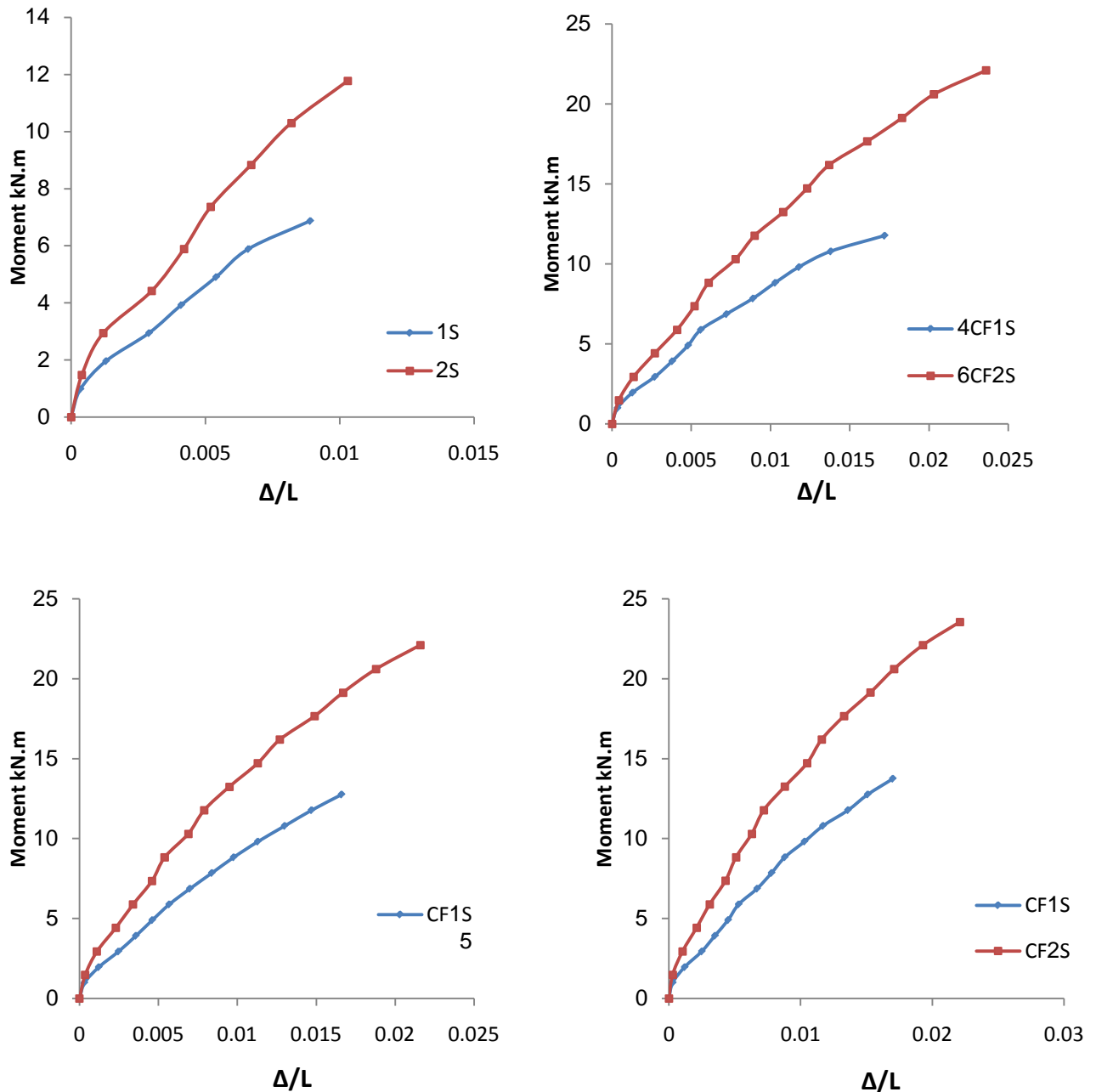
Fig. (10): Moment-midspan deflection-to-span ratio curves for sand-PLWAC OWS.
