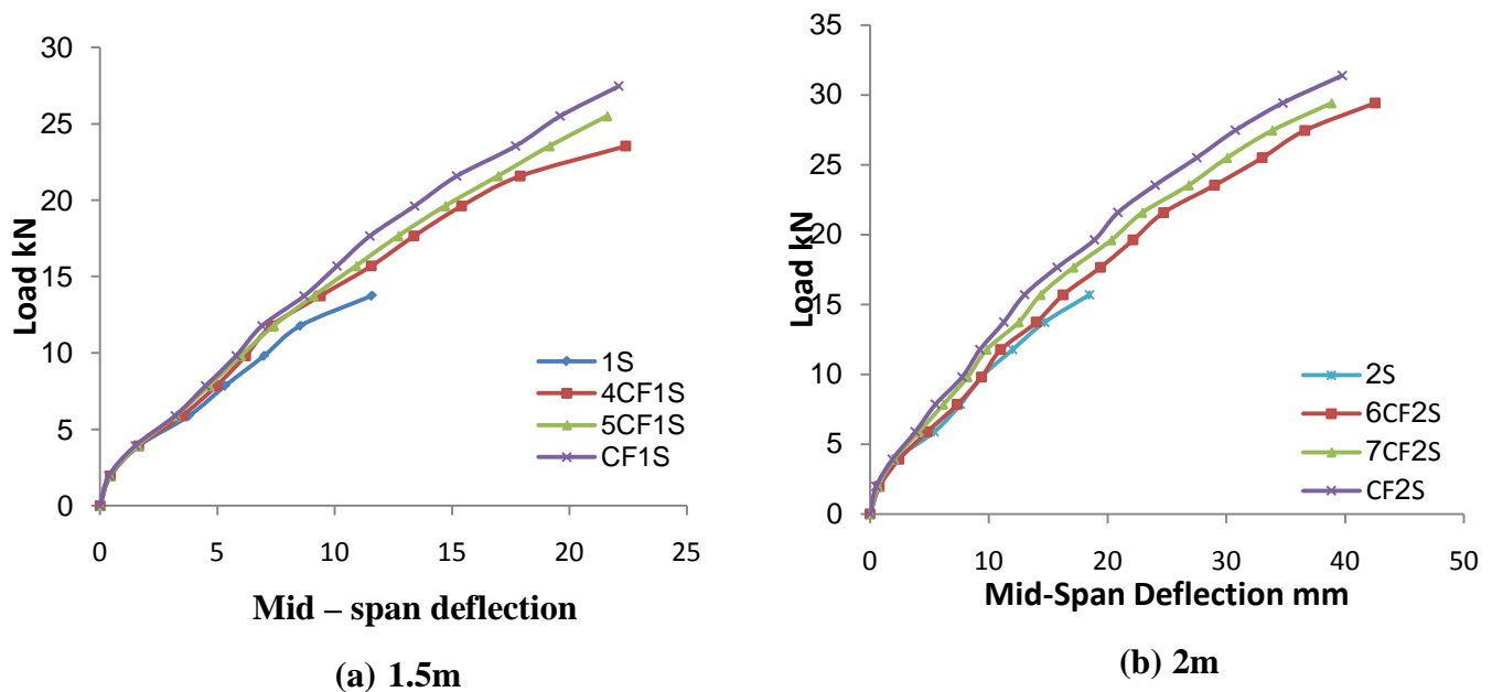
Fig. (8): Load – midspan deflection curves.
