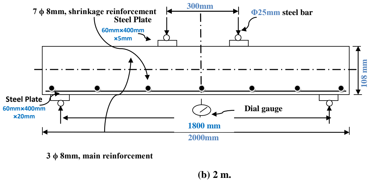
Fig. (4): Dimension, Loading, Reinforcement
