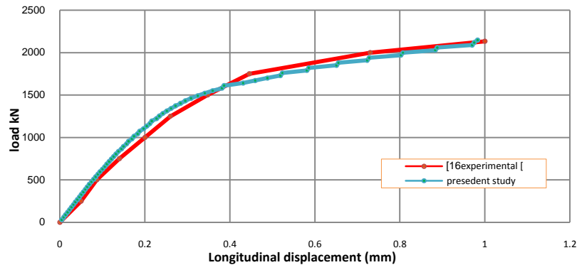
Fig. (9):Experimental and numerical load-longitudinal displacement for column specimen (C1-1).
