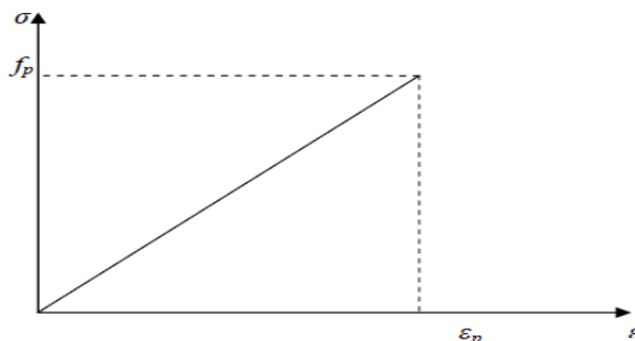
Fig. (8) : Stress-strain Relation of CFRP [7]
